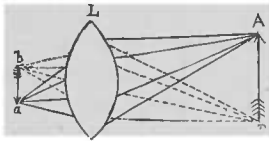
FIG. 129.—Diagram illustrating the formation of an image by a converging lens.
