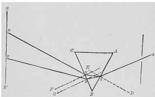
FIG. 128.—Diagram illustrating the dispersion of mixed light by a prism.
