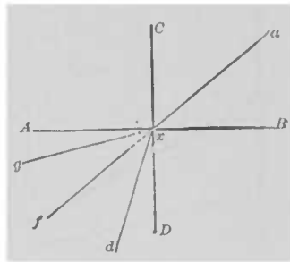
FIG. 127.—Diagram illustrating the refraction of light. AB , surface of separation between two transparent media; CD , the perpendicular to the surface at the point of incidence, x ; ax , incident ray; xd , refracted ray, if the second medium be denser than the first; xg , refracted ray, if the second medium is less refractive than the first. The reflected ray is not represented, but would make an angle with Cx equal to the angle axC .
